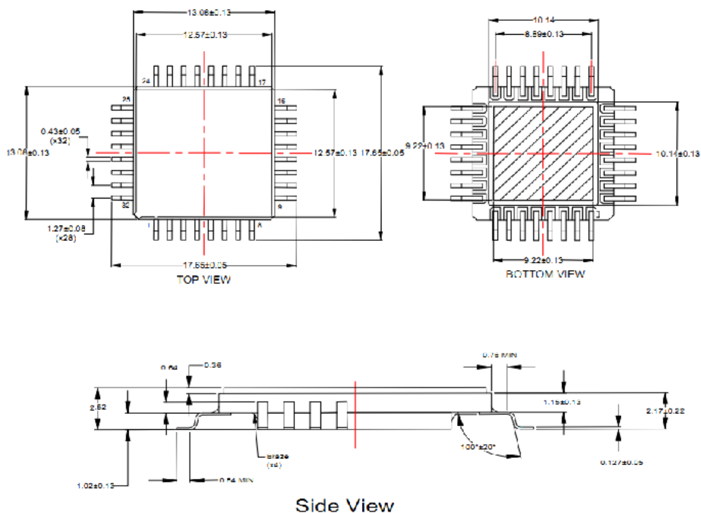
Figure 13. Package Drawing 32-lead CQFP
