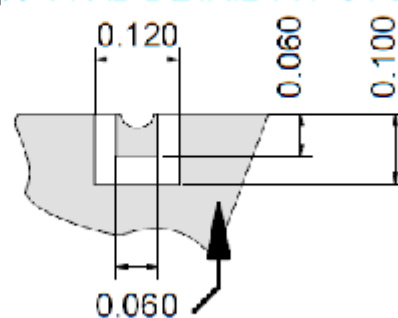
Type 1 PAD DETAIL TYP 3 PLCS.
