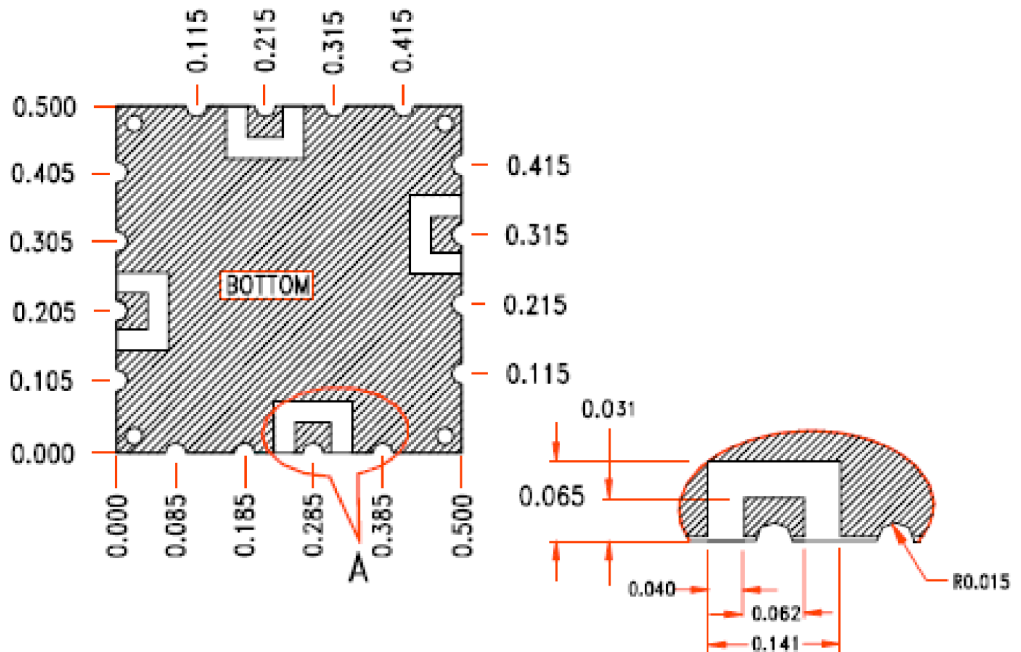
DETAIL-A
