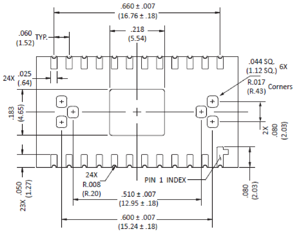
Bottom View
