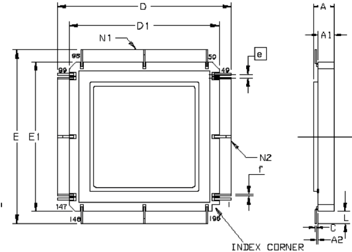
Figure 5-1. MQFPF 196 package
