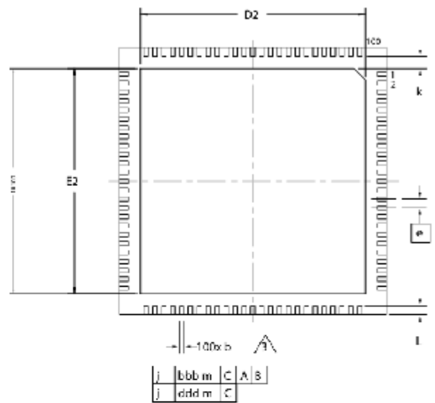
BOTTOM VIEW PACKAGE FLIPPED LEFT TO RIGHT
