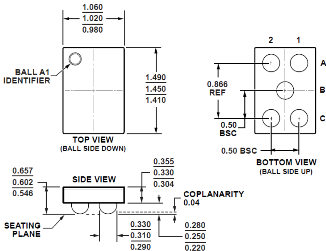
Figure 36. 5-Ball Wafer Level Chip Scale Package [WLCSP] (CB-5-3)
